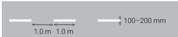
Figure 4.15 – Dashed White Bicycle Lane Line
