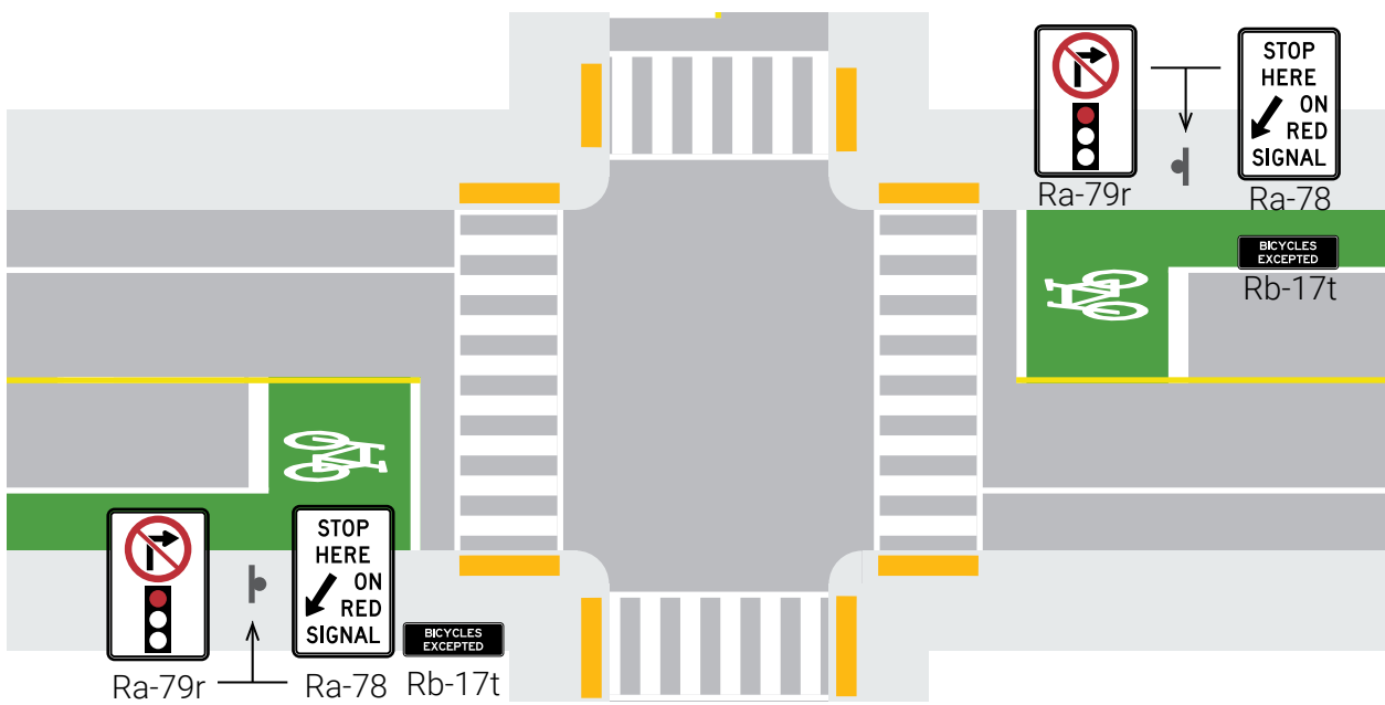
Figure 6.55 – Bike Box, Typical Intersection
