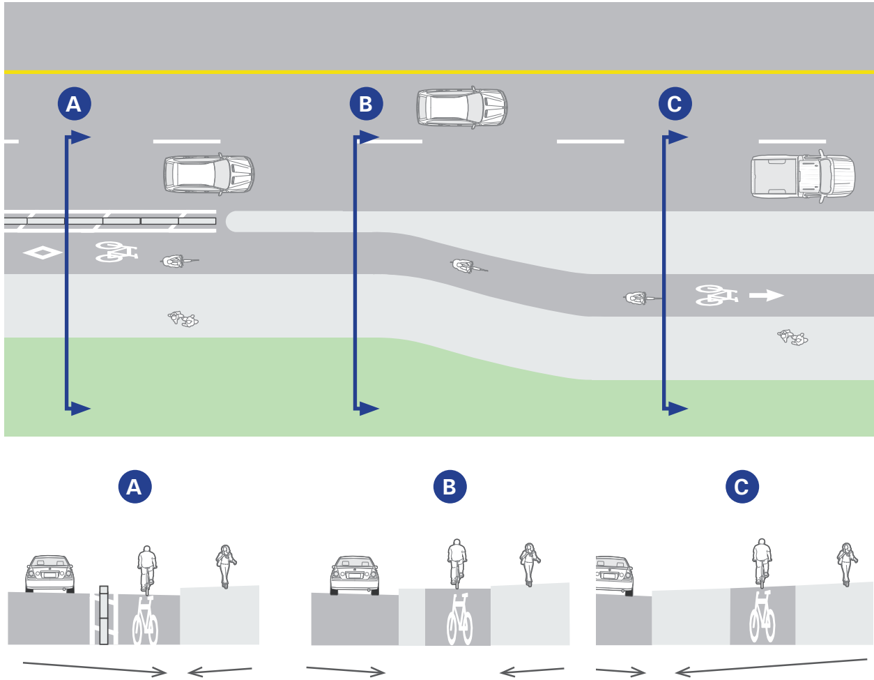
Figure 6.65 – Transition Between On-Road and In-Boulevard Facility
