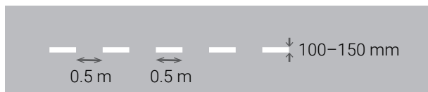
Figure 6.6 – Condensed Dashed Guide Line
