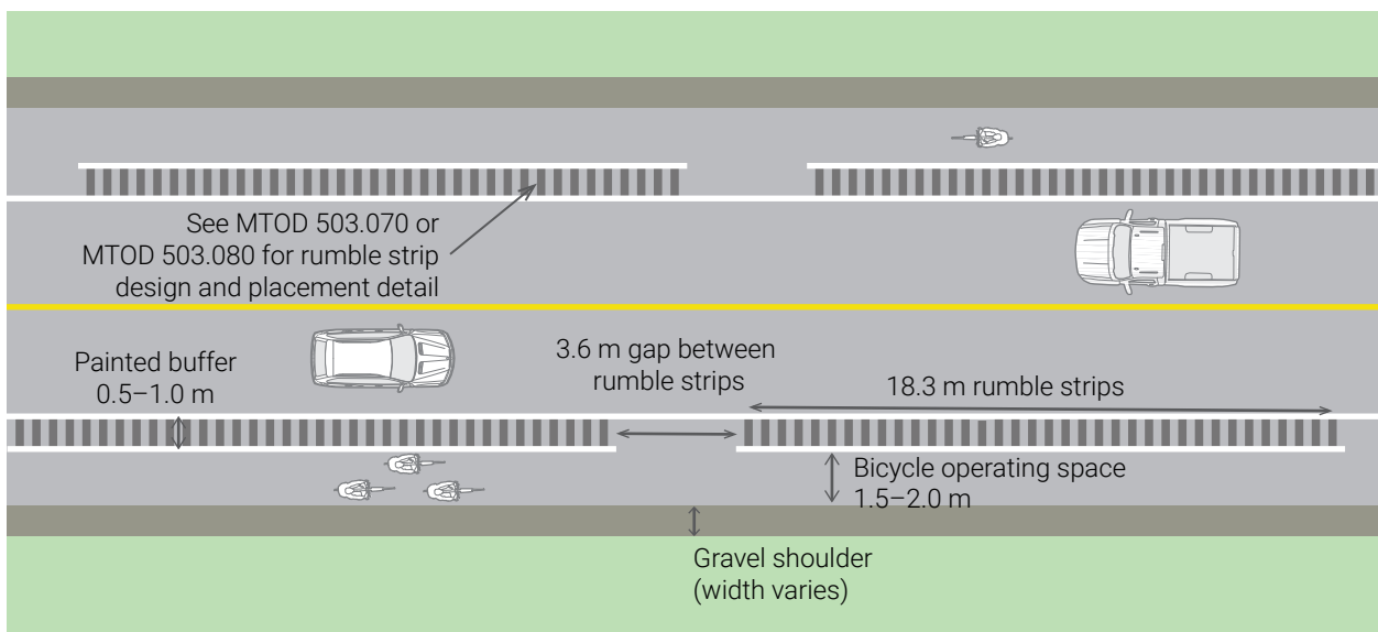
Figure 4.75 – Paved Shoulders with Rumble Strips
