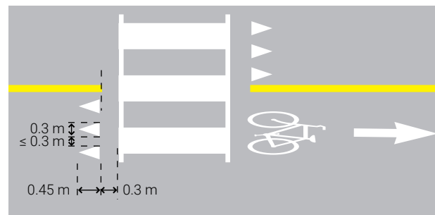
Figure 6.8 – Yield Line on Cycling Facility
