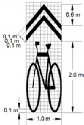
Figure 4.18 – Shared Use Lane (Sharrow) Pavement Marking
