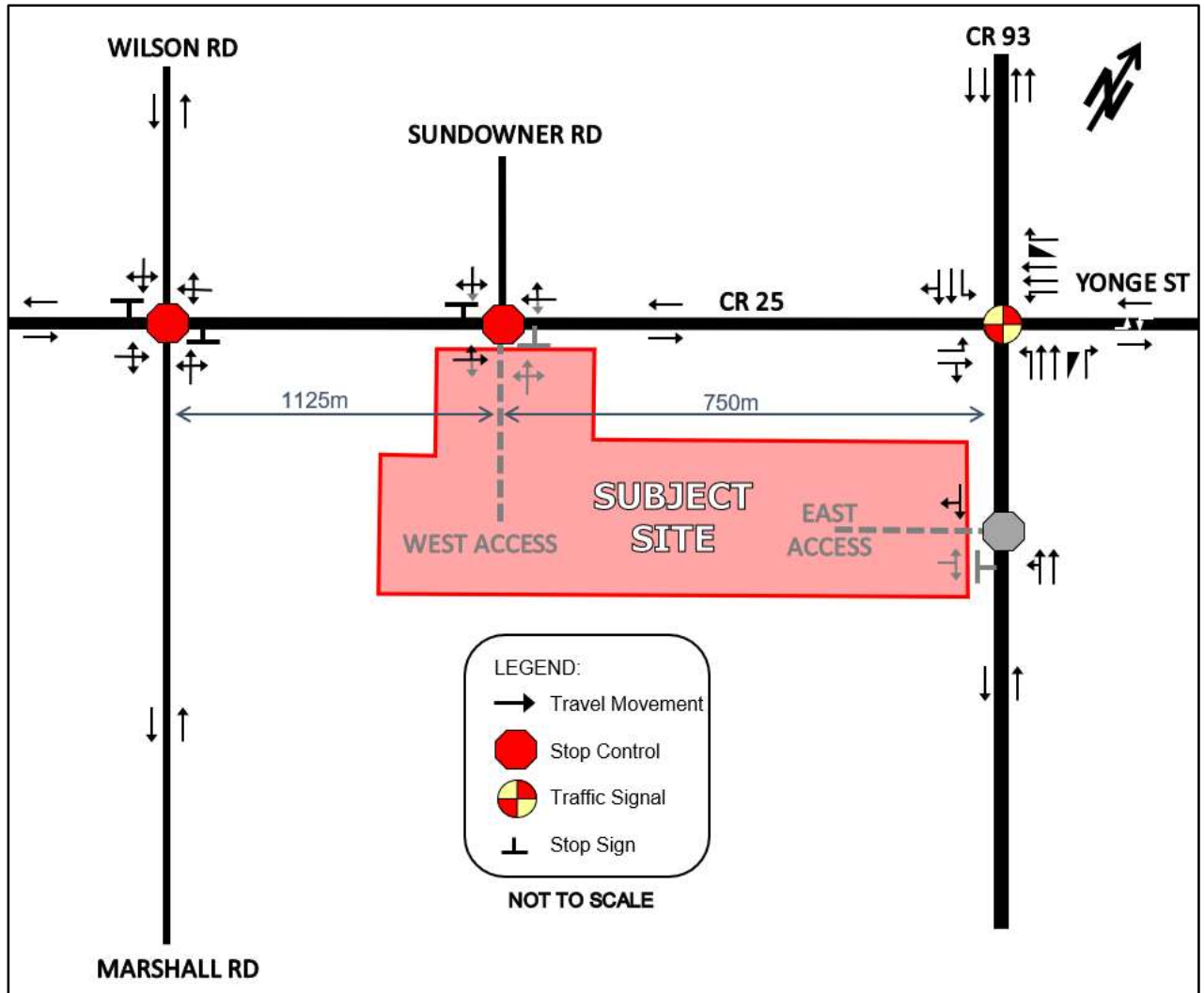
Figure 2 – Existing Intersection Lane Configuration within Study Area
