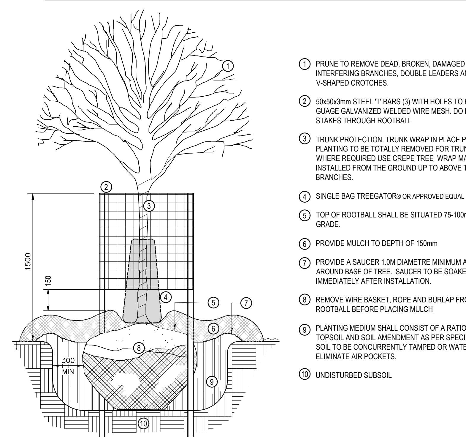
1 DECIDUOUS TREE PLANTING Section
